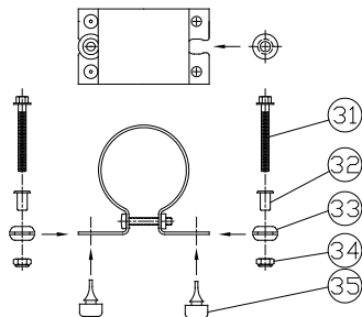
FIGURE 2 BRACKET ASSEMBLY
