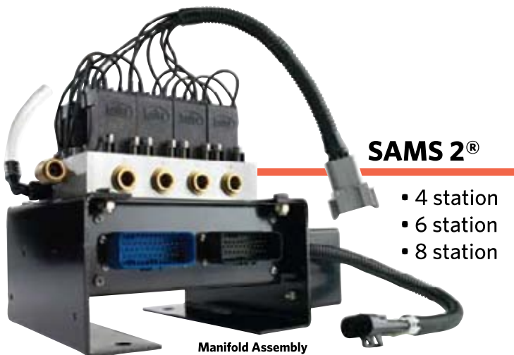
Manifold Assembly
